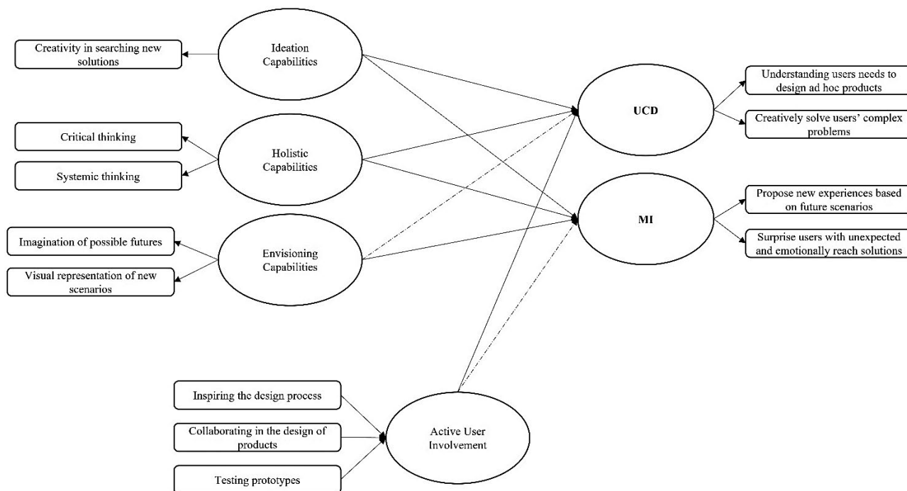
FIGURE 1 Complete structural equation model
